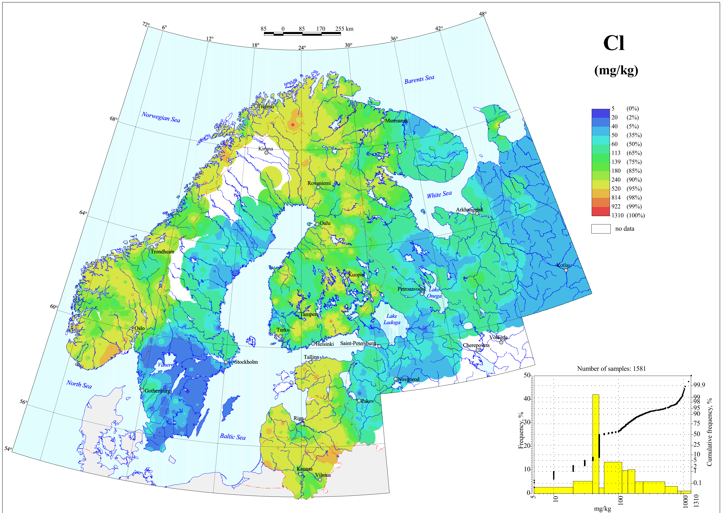
Chloride in C-horizon, Grain Size <2 mm, Total Content
